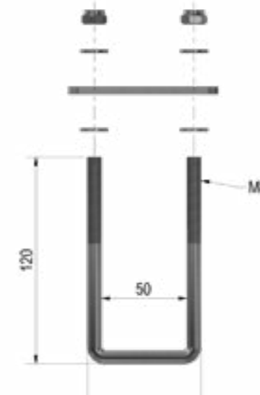
With this mounting set it is possible to mount a box on a drawbar.
